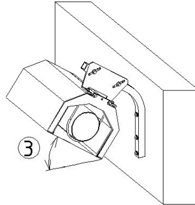
SUPPORT MURAL
