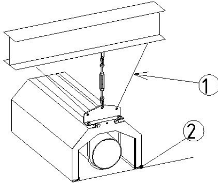
SUPPORT HORIZONTAL
