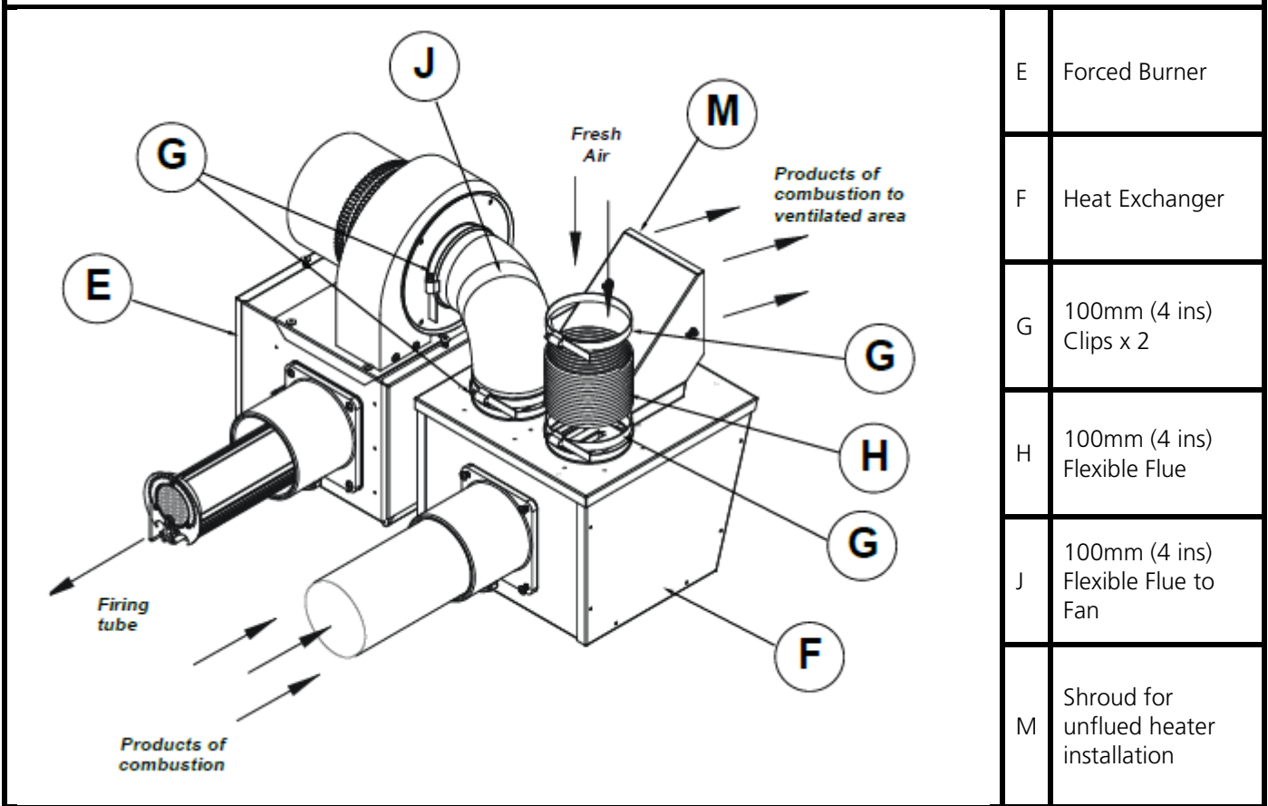
Diagram 2 Forced Burner with Heat Exchanger (No External Flue) for ducted air and products of combustion to ventilated area
