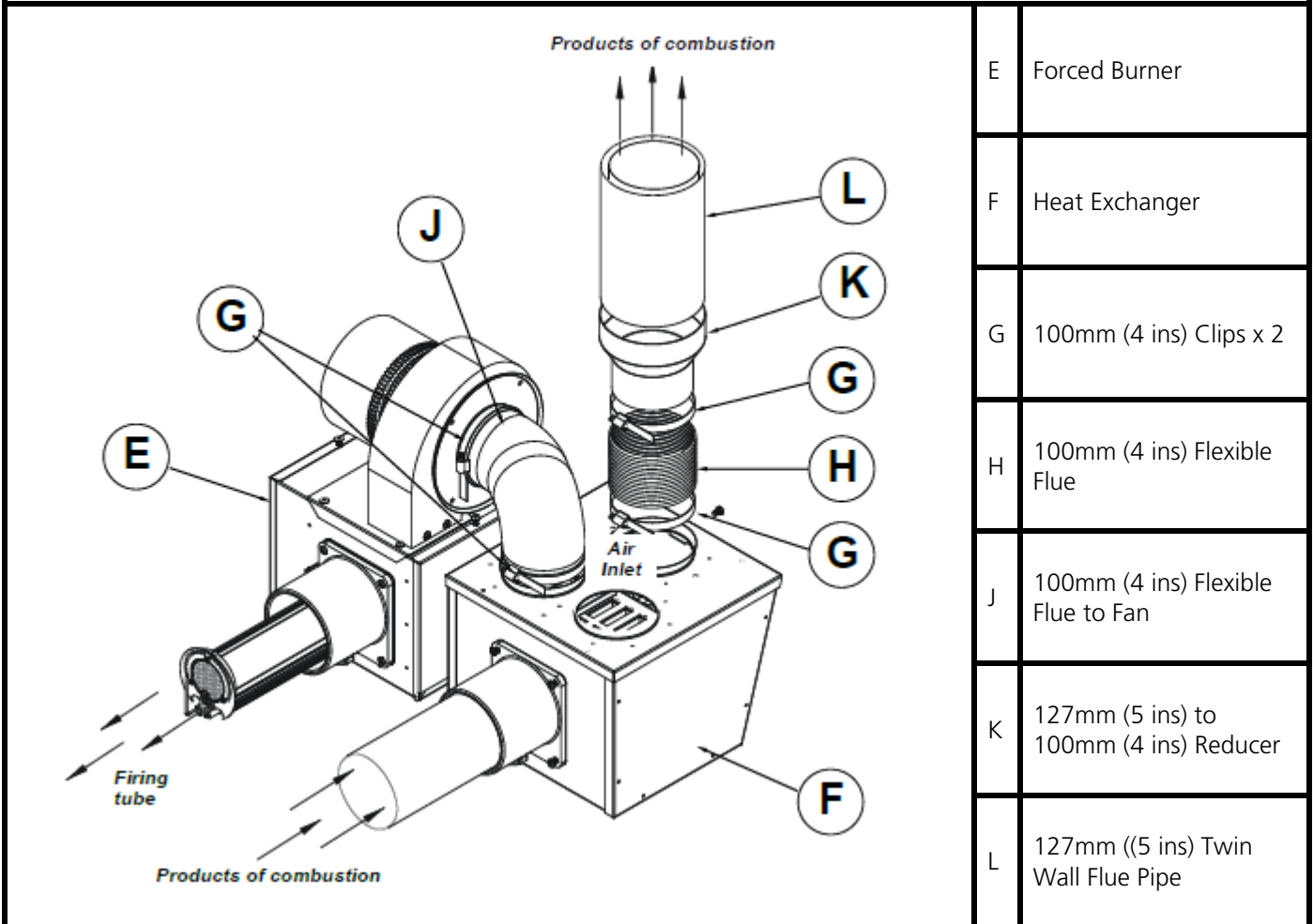
Diagram 1 Forced Burner with Heat Exchanger (Standard Flue) for flue products of combustion and no ducted air
