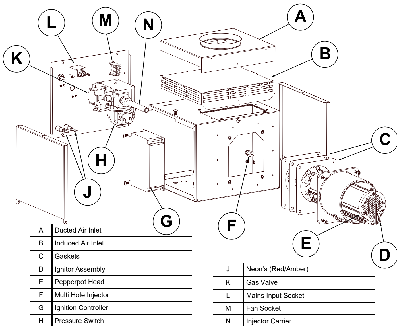
Figure 20. Induced Herringbone Burner: Model VSO UT/UH (refer to spares section 5)
