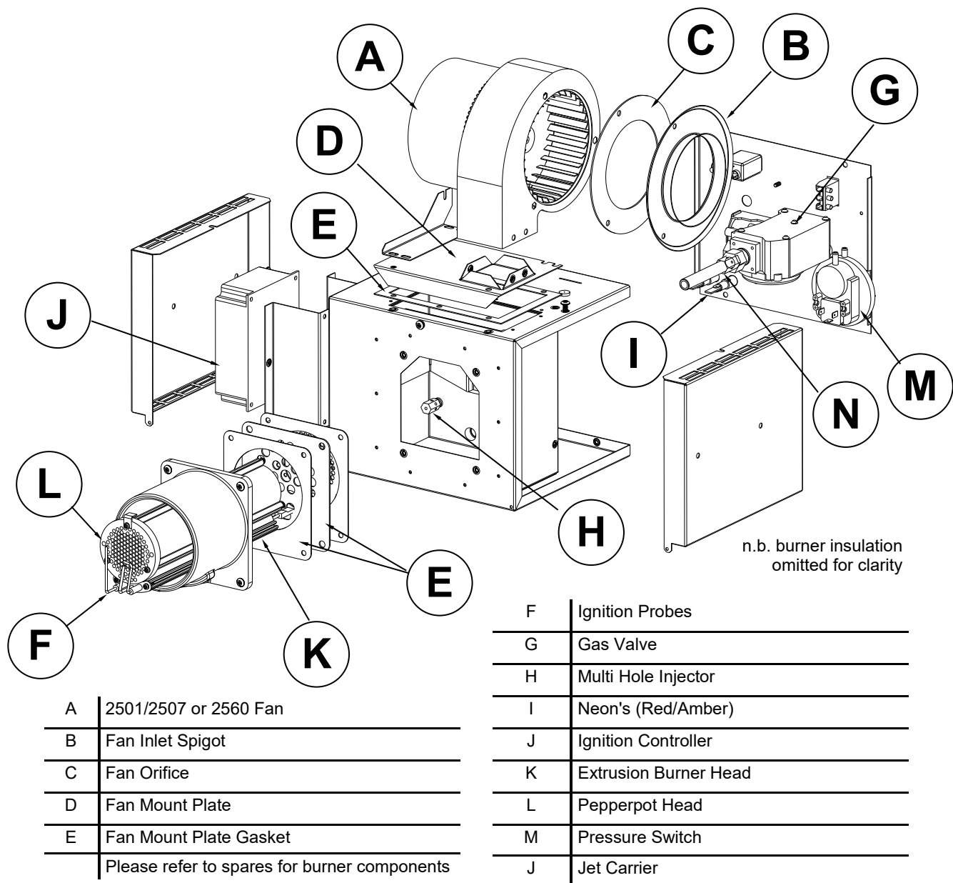
Figure 21. Forced Gas Burner: Model VSXO (refer to spares section 5)
