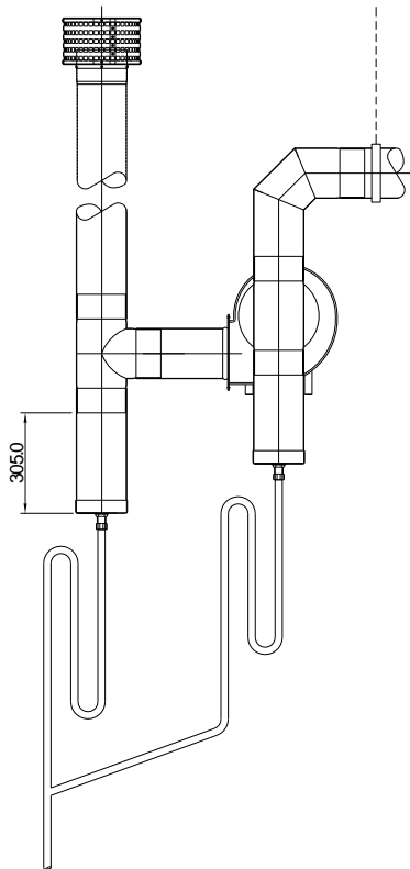
Figure 2f. Conventional Flue Arrangement Wall Exit.
