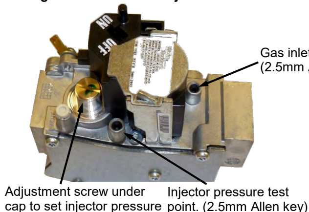
Figure 19. Gas Valve adjustment
