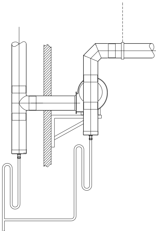
Figure 2g. Stainless Steel Telescopic Through The Wall Arrangement (available
