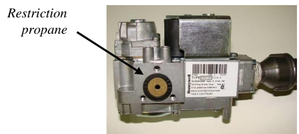
Figure 15 : Propane
