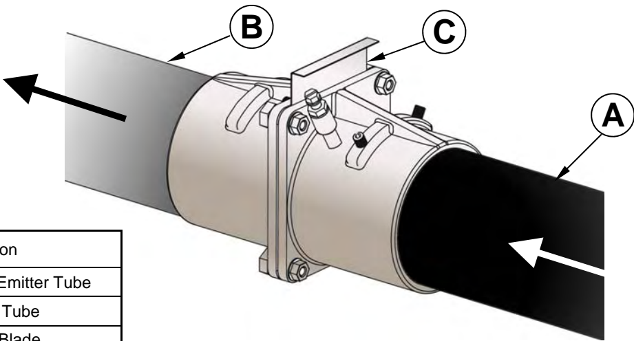
Figure 18. HB Damper Assembly
