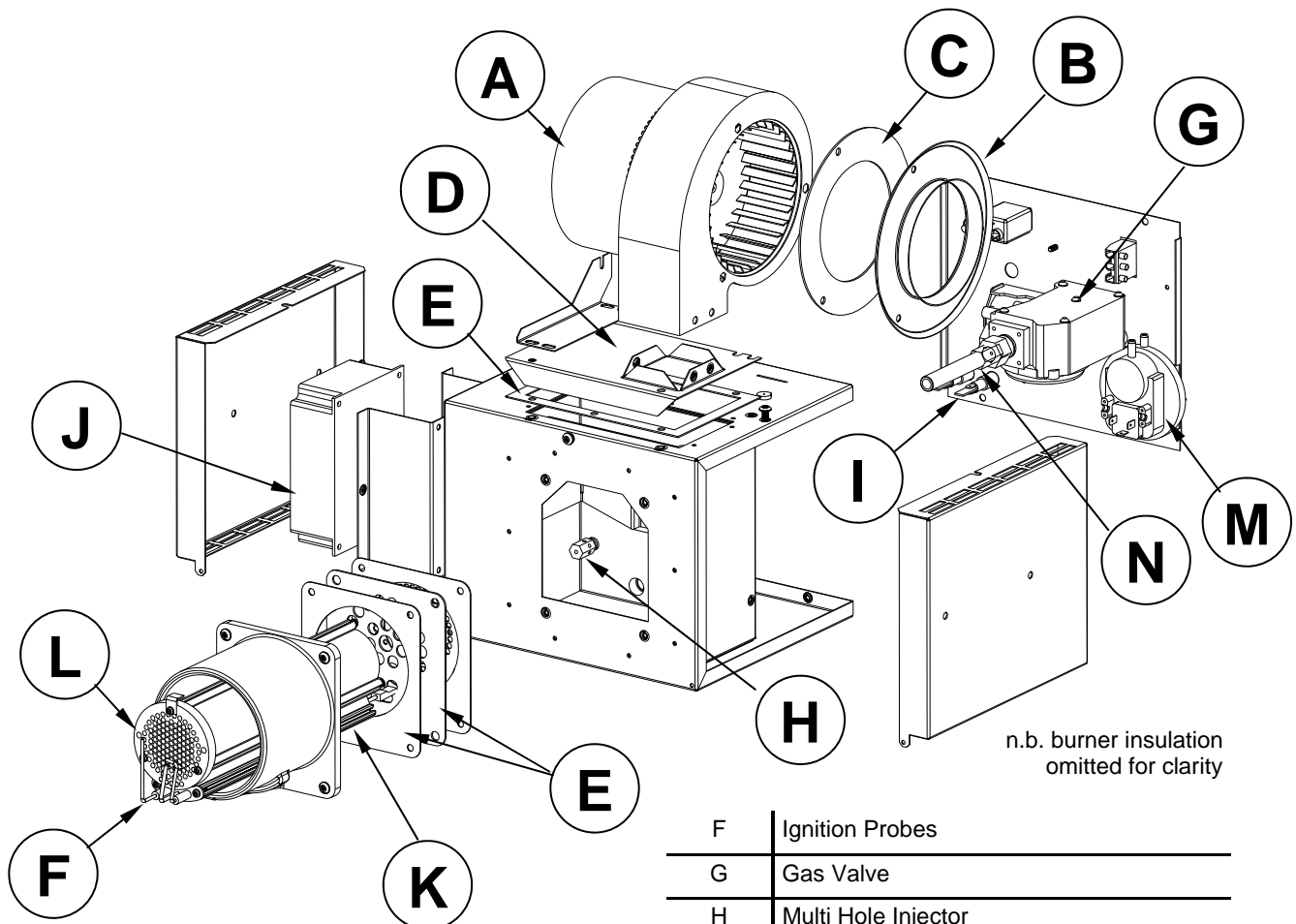
Figure 21. Forced Gas Burner: Model VSXO (refer to spares section 5)
