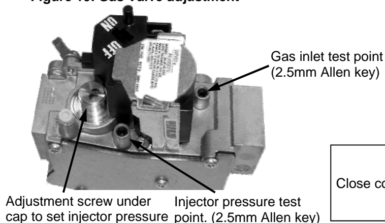
Figure 19. Gas Valve adjustment
