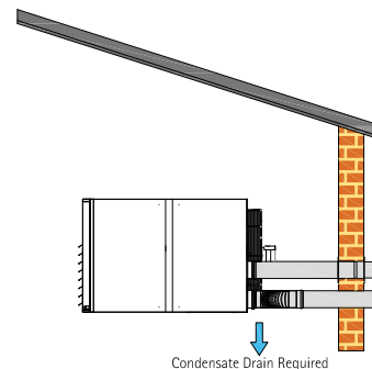
Separate combustion air and flue pipes (type C12) for applications where wall thickness exceeds 350mm. Flue and air intake to be offset
