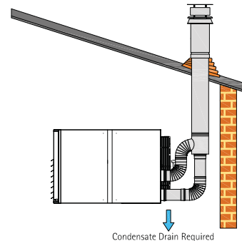
Balanced flue roof outlet (type C32)
