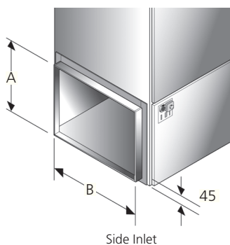
Side Inlet
