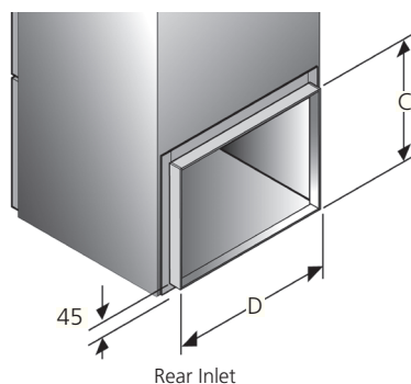
Rear Inlet
