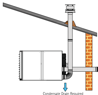
Combustion air through the wall, flue outlet through the roof (type C52)
