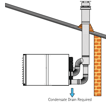
Balanced flue roof outlet (type C32)
