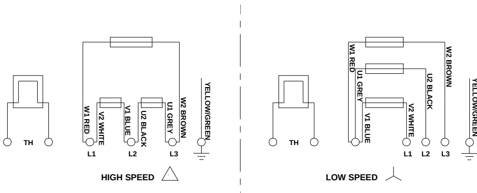
Diagram 6. Motor speed options
