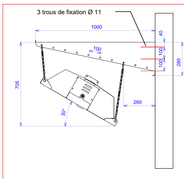
SUPPORT MURAL
