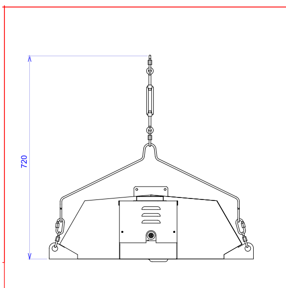
SUPPORT HORIZONTAL
